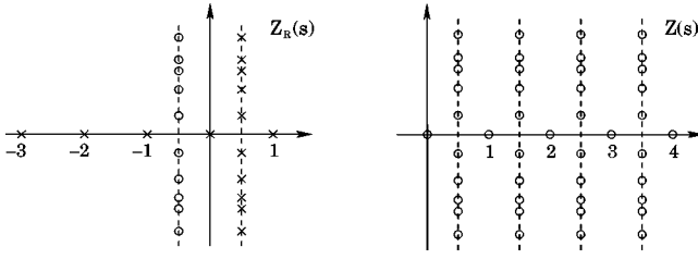
FIG. 1. Analytic structure close to the origin of the Ruelle zeta function (left) and of the spectral determinant (Ruelle-Pollicott resonances, right) for a compact and closed billiard on a surface of constant negative curvature. Crosses are poles, circles are zeros. Multiplicities and exact positions are given in the text.
